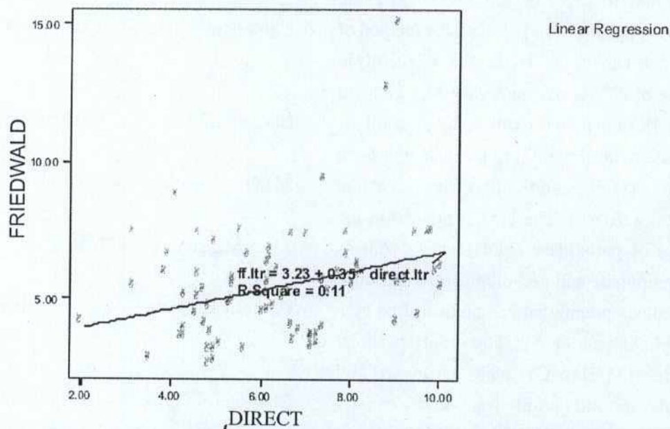
Figure 1: Linear Regression Analysis of LDL-C Estimation by Friedwald's Formula and Direct Method
