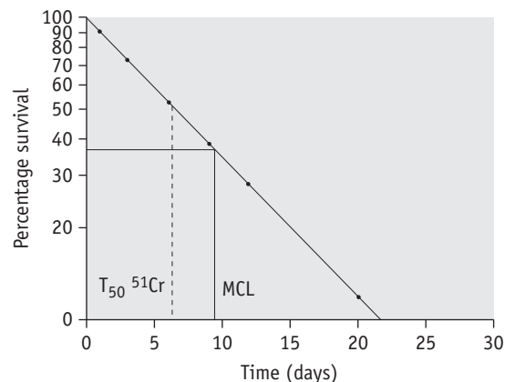
Figure 17.7 ^{51}\text{Cr} red cell survival curve. Patient with autoimmune haemolytic anaemia. The results have been plotted on semilogarithmic graph paper and the mean cell lifespan was read as the time when 37% of the cells were still surviving (9–10 days). The T_{50}\text{Cr} was 6–7 days. MCL, mean cell lifespan.
