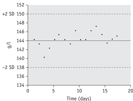
Figure 25.2 Control chart for haemoglobinometry by manual method. The limits for satisfactory performance have been set at \pm 2SD .
