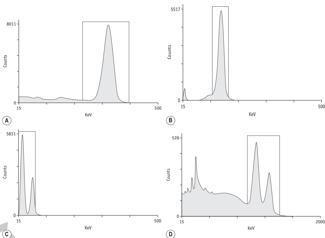
Figure 17.1 Spectra of radioisotopes obtained on a scintillation spectrometer. (A) ^{51}\text{Cr} , (B) ^{99\text{m}}\text{Tc} , (C) ^{125}\text{I} and (D) ^{59}\text{Fe} . The radionuclides should be counted with the window set within the limits indicated by the vertical lines.
