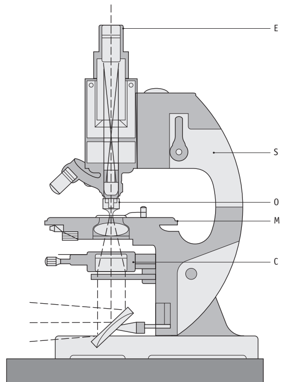
Figure 3.9 Cross-section of microscope, showing its components. E, eyepiece; S, stand; O, objective; M, mechanical stage; C, condenser. The broken lines indicate the light path. Note that this shows an external light source being directed into the microscope. In most modern microscopes there is a built-in lamp in the base.
