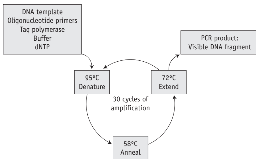
Figure 8.1 The polymerase chain reaction. Cyclical repetition of three temperatures for denaturing, annealing and extending DNA, respectively, gives rise to an exponential amplification of a DNA fragment between two primer sequences directing DNA synthesis on opposite strands of the DNA template.
