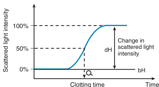
Figure 18.2 Endpoint determination: percentage detection method.
