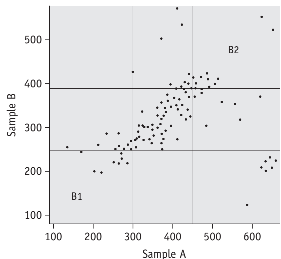
Figure 25.5 Youden (xy) graph. The range of standard deviations (SDs) calculated from the overall results with sample x and sample y, respectively, are drawn on the x axis and the y axis; the individual paired results are then plotted on the graph. Results in the central square are satisfactory; those in B demonstrate a consistent bias with measurements that are too low (B1) or too high (B2), whereas results in other areas indicate random errors (inconsistency) in the two samples.
